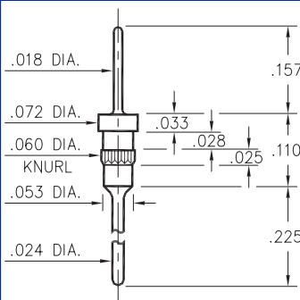
5011-0-00-XX-00-00-03-0 Press-fit in .057 mounting hole
